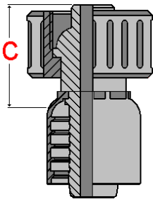
P23.6213 Brass Metric Female with Plastic Handle (Kaercher type)
